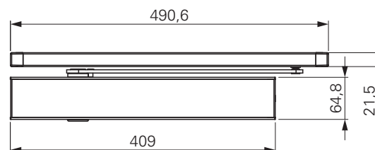
Dimensioner: ECO FTS III
